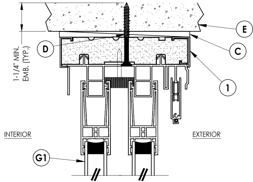
3 3 VERTICAL CROSS SECTION Shown w/ Direct to Masonry option
